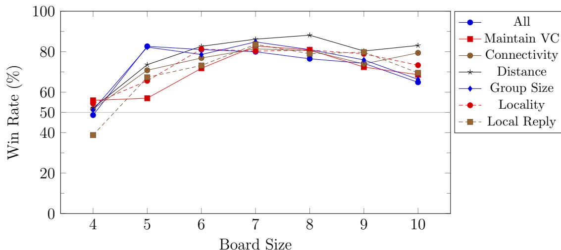
Figure 4.26: Knowledge Modifications
