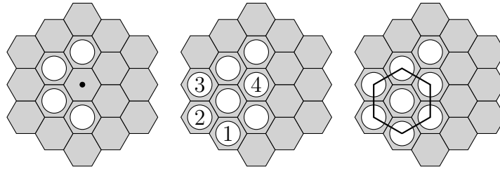
Figure 3.6: Hex-dead Cells Are Not Havannah-dead Cells. Starting with the Hex-dead cell pattern on the left, and adding stones 1-4 leads to the ring on the right which intersects the Hex-dead cell
