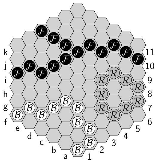
Figure 3.1: The Three Havannah Winning Conditions, as shown on a size 6 Havannah board
