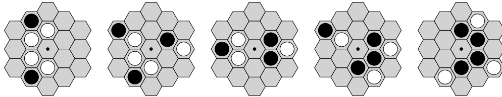
Figure 3.7: Some Havannah Dead Cell Patterns. The cells marked with the dot are dead in Havannah.
