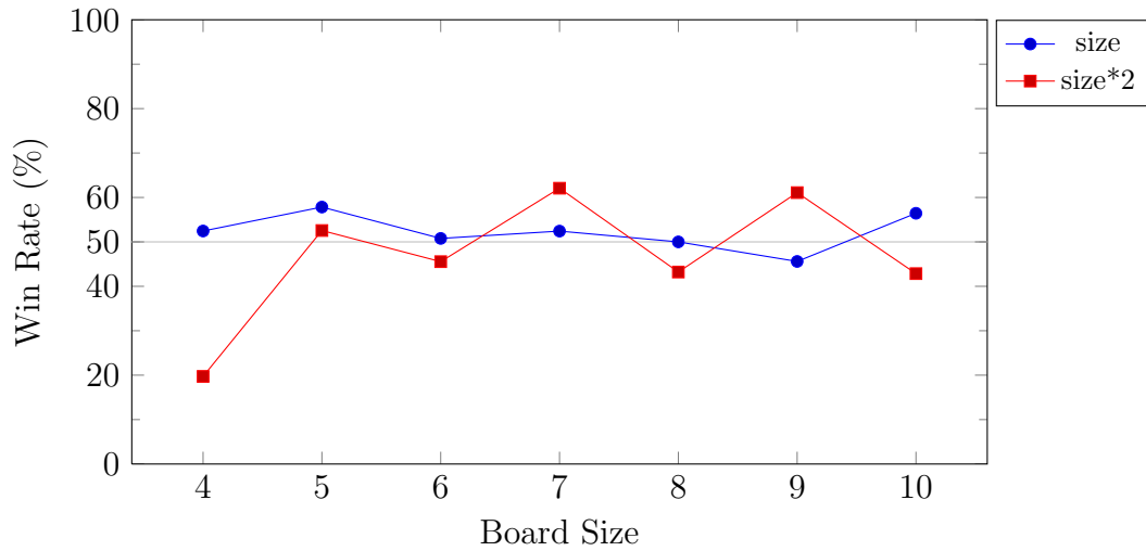
Figure 4.18: Mate-in-one Checking Against Baseline RAVE Player With 30 Seconds per Move
