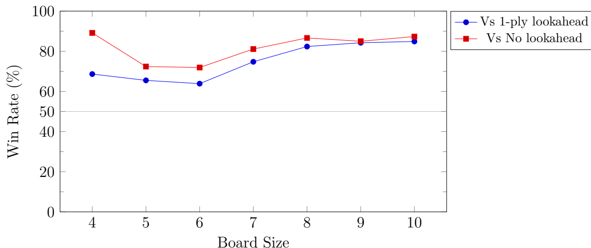
Figure 4.5: RAVE Baseline with 2-ply lookahead during expansion vs 1-ply lookahead and no lookahead
