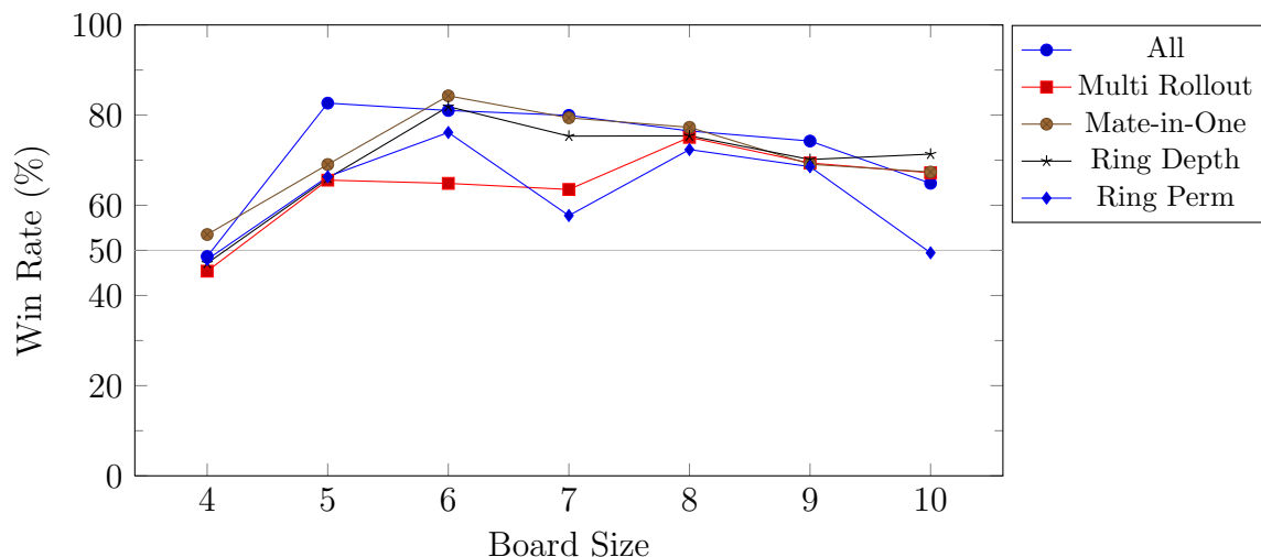
Figure 4.25: Rollout Modifications
