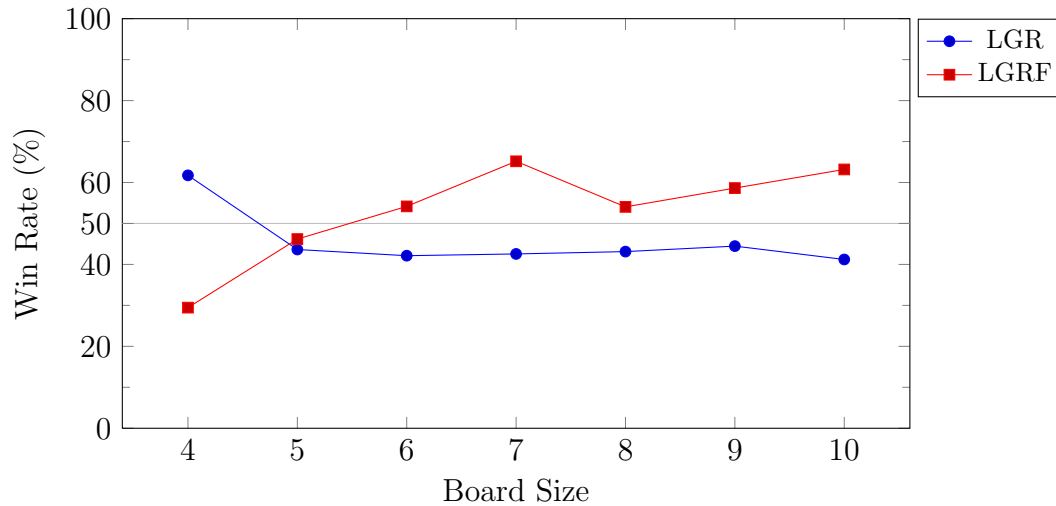
Figure 4.20: Last Good Reply Against Baseline RAVE Player
